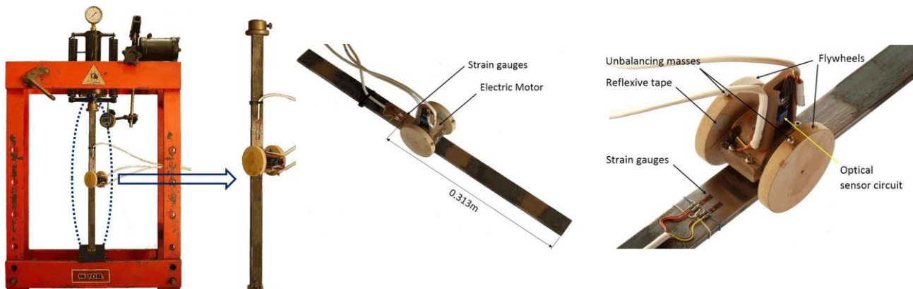
Figure 1: The experimental setup
